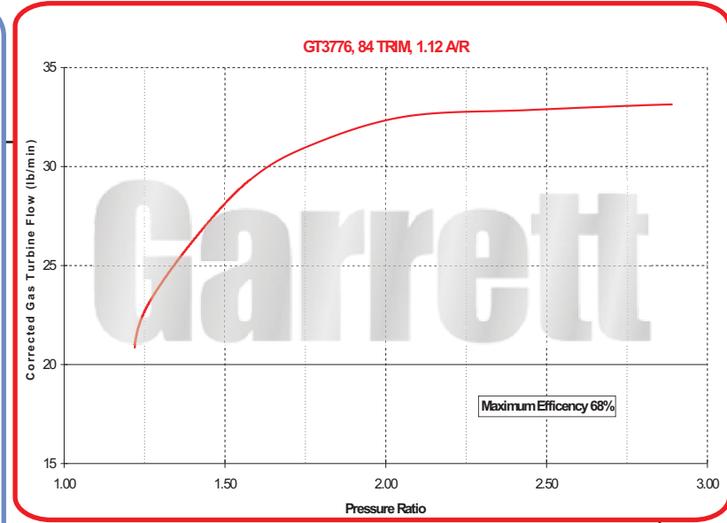
Turbine Map
