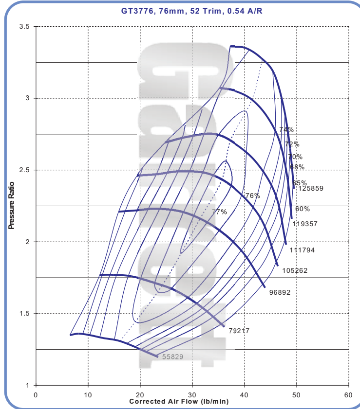
Compressor Map
